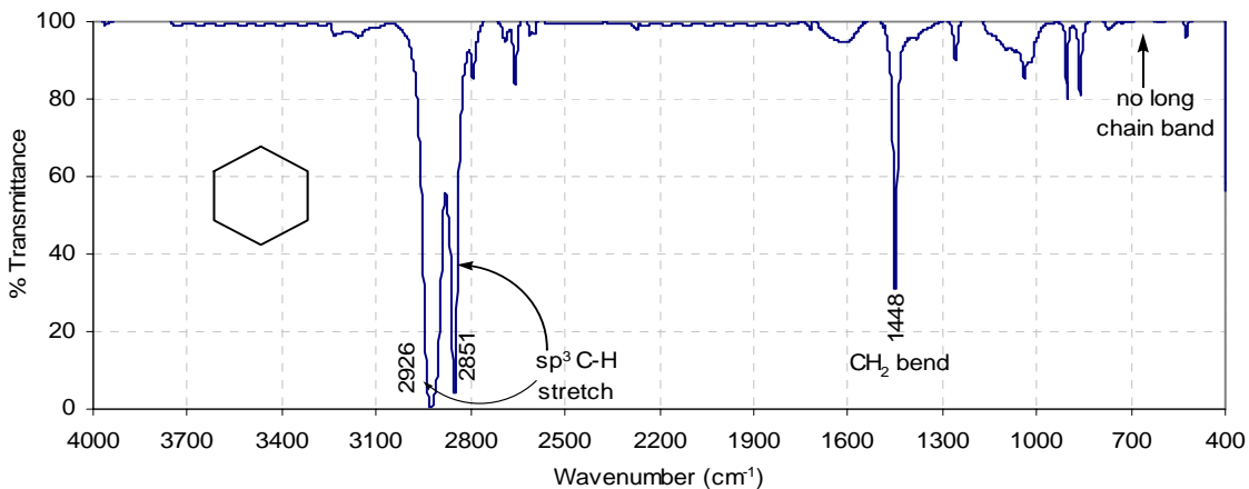
Figure 15 : The infrared spectrum of cyclohexane (neat liquid)
