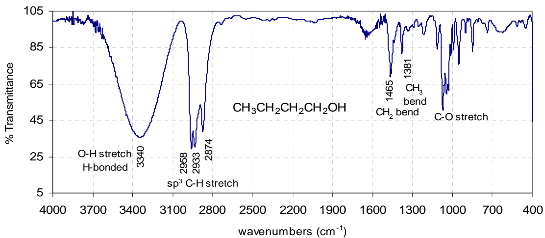
Figure 21 : The infrared spectrum of 1-butanol (neat liquid)
