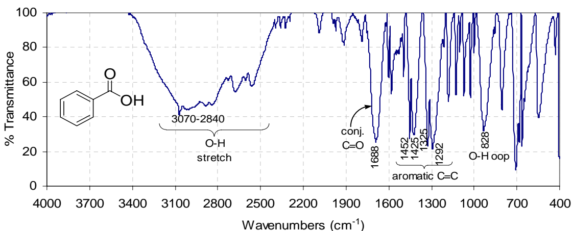
Figure 33 : The infrared spectrum of benzoic acid (nujol mull)
