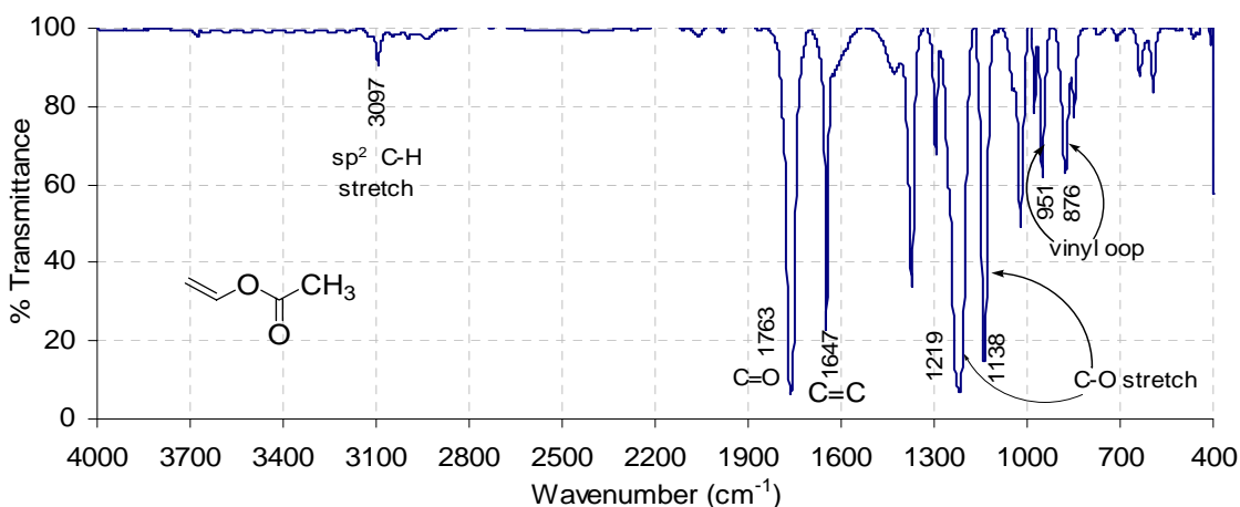
Figure 36 : The infrared spectrum of vinyl acetate (neat liquid)
