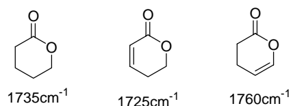
Figure 34 : Effect of conjugation in cyclic esters
