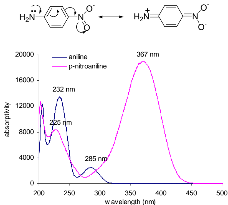
Figure 11 : UV-spectra of aniline and p -nitroaniline in methanol
