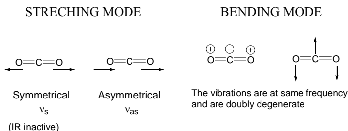
Figure 13: Vibrational modes for carbon dioxide molecule
