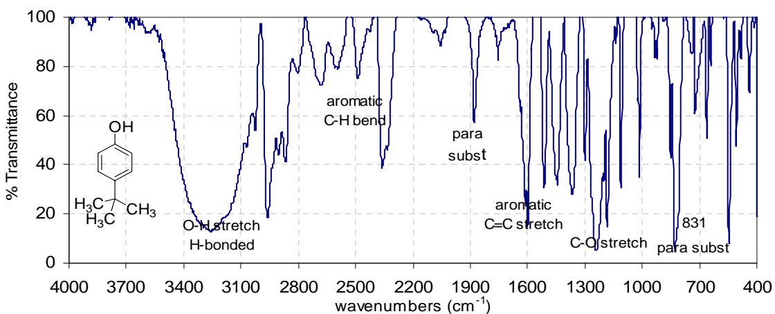
Figure 22 : The infrared spectrum of t-butylphenol (nujol mull)
