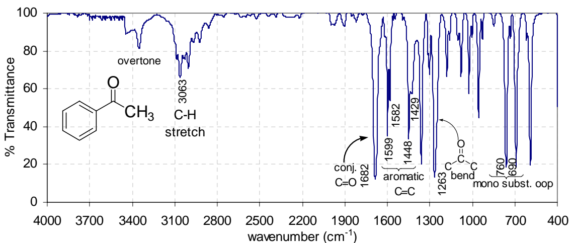
Figure 31 : The infrared spectrum of acetophenone (neat liquid)
