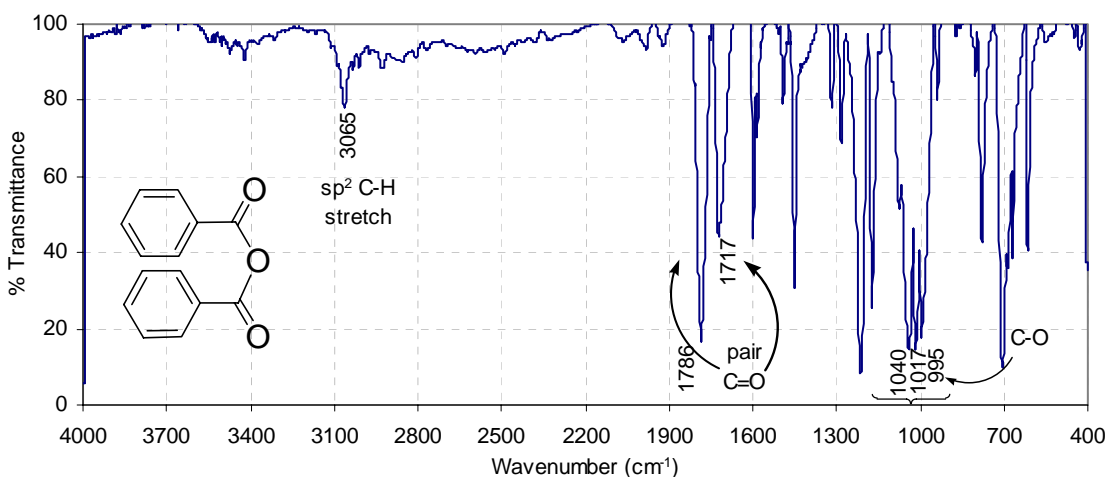
Figure 37: The infrared spectrum of benzoyl anhydride (nujol mull)
