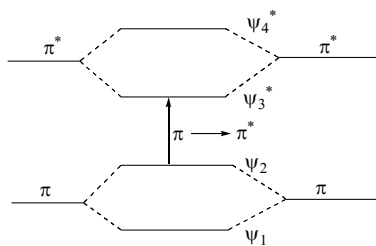
Figure 6 : Effect of conjugation on orbitals' energy and respective \pi - \pi^* transition.
