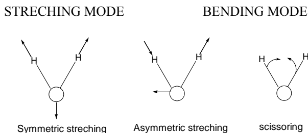
Figure 12: Vibrational modes for water molecule
