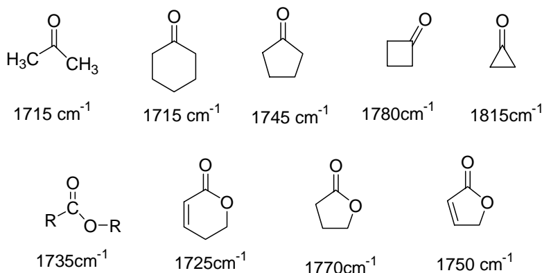
Figure 28 : C=O stretching frequencies in various compounds
