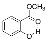
methyl salicylate
