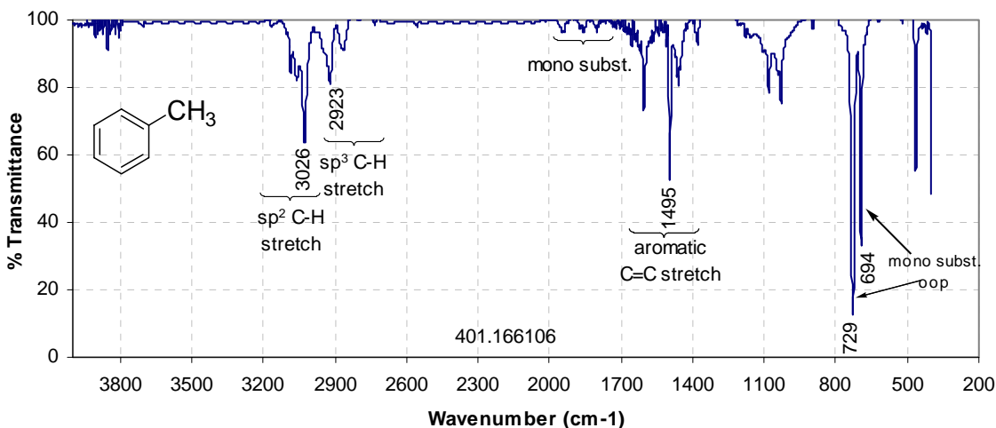
Figure 18 : The infrared spectrum of toluene (neat liquid)
