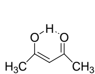
acetyl acetone
