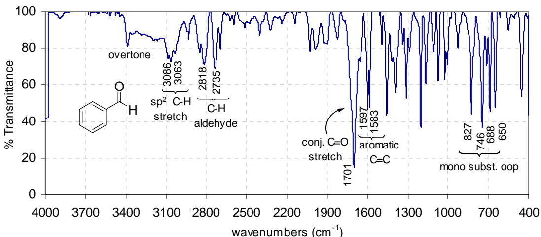
Figure 30 : The infrared spectrum of benzaldehyde (neat liquid)
